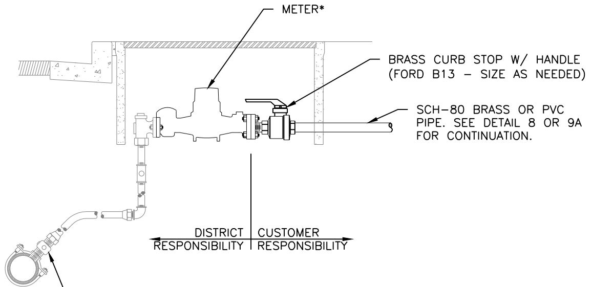
ELEVATION VIEW
